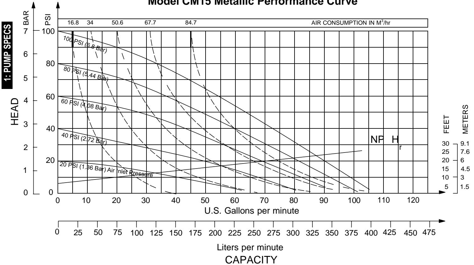
Model CM15 Metallic Performance Curve
